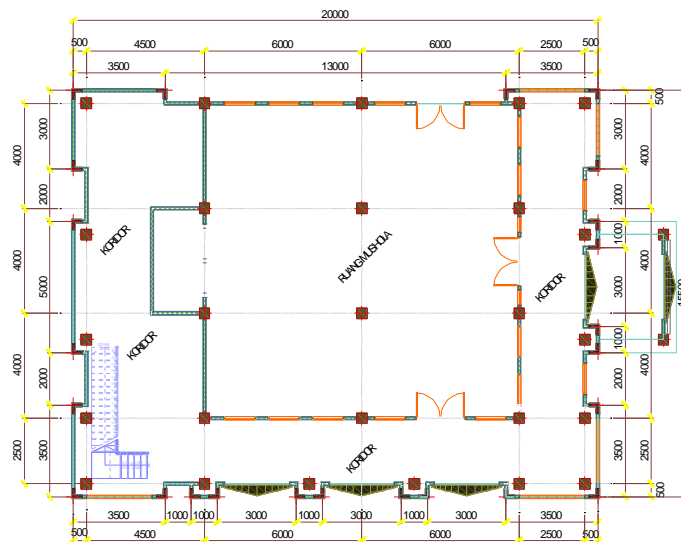
Gambar 3. Denah Lantai 1
